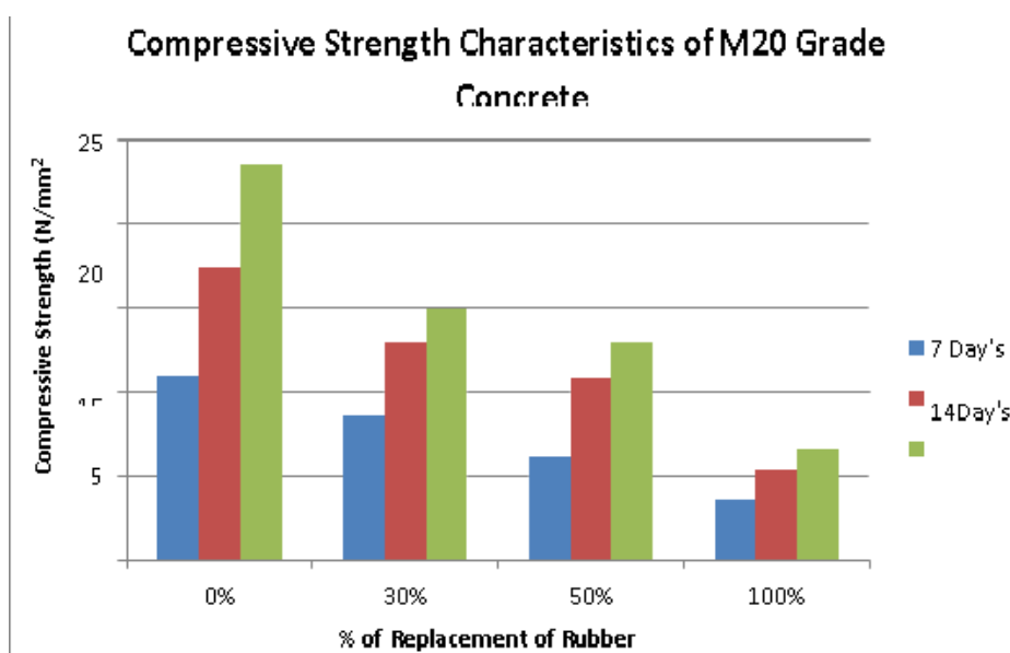
GRAPH : 2 Percentage of Replacement of Rubber V/s Compressive Strength of M20 Concrete :
